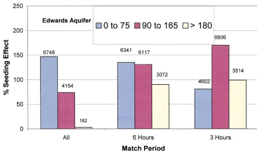
FIG. 7. Apparent seeding effect (%) as a function of pretreatment age at initial treatment and match period for matches made outside the operational target for the Edwards Aquifer program in 1999, 2000, and 2001. The average rain change (acre-feet) per unit is shown above each bar.
